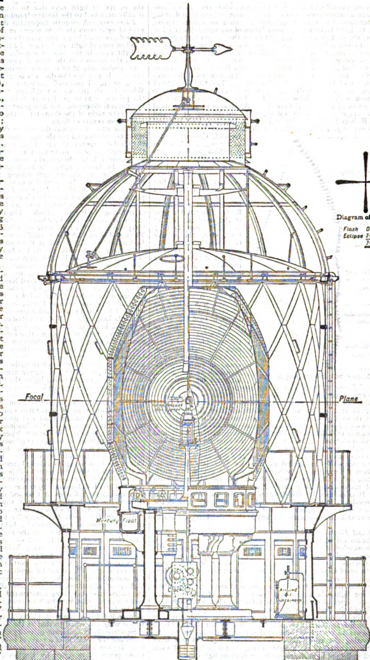
FIG. 41.—Manora Point Apparatus and Lantern.
