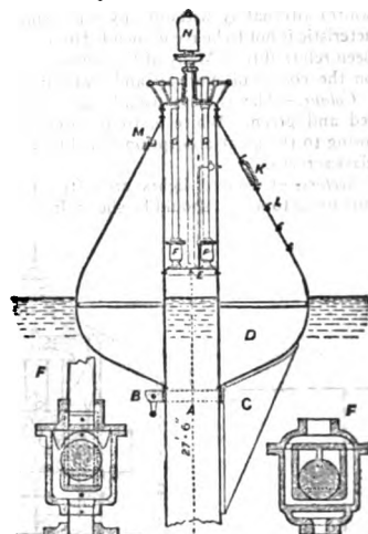
FIG. 51.—Courtenay's Automatic Whistling Buoy.
