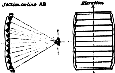
FIG. 37.—Chance's Dioptric Spherical Mirror.
