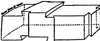
FIG. 23.—Perspective drawing of Dovetailed Stone (Wolf Rock).
