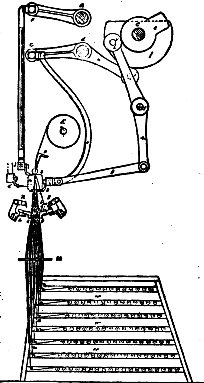
FIG. 49.—Section of Lace Machine.
