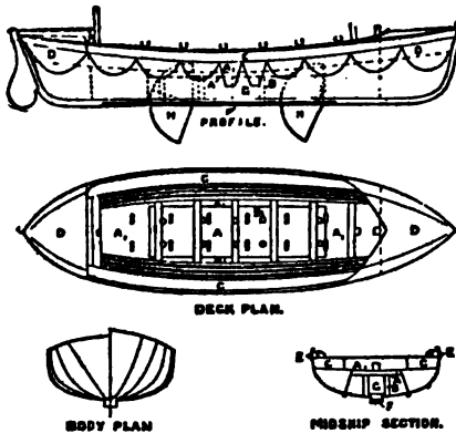
FIG. 8.—Plans and Section of Watson Type of Life-boat. Lettering as in fig. 5, but C, side air-cases above deck and thwarts.
