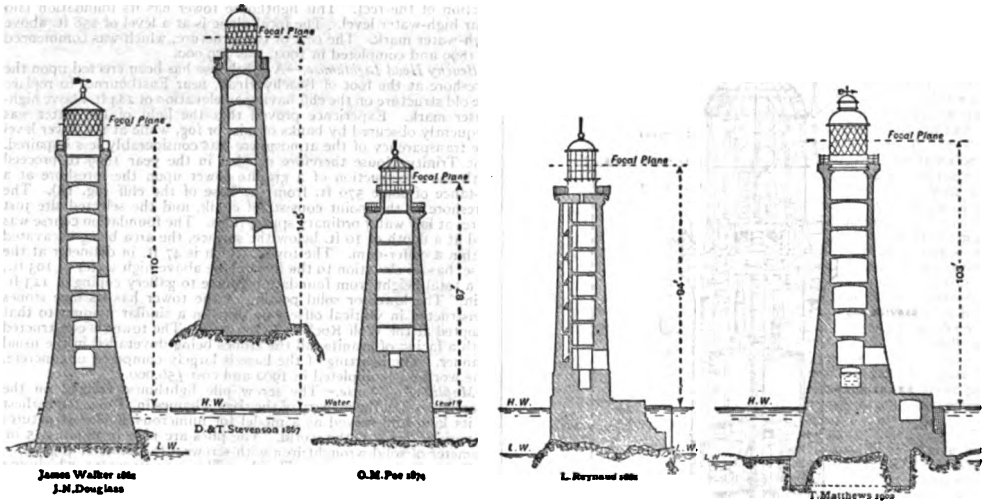
FIG. 14.—Wolf Rock. FIG. 15.—Dhu Heartach. FIG. 16.—Spectacle Reef. FIG. 17.—Ar men. FIG. 18.—Beachy Head.
