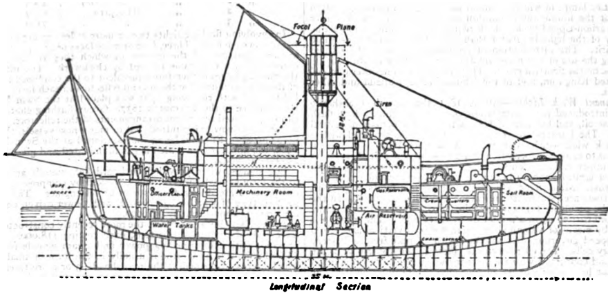
FIG. 47.—Sandetti Lightship.
