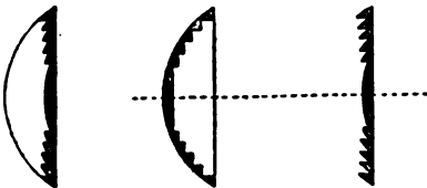
FIG. 31.—Buffon's Lens.
