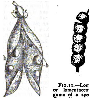
FIG. 10.—Dry dehiscent Fruit. The pod (legume) of the Pea.
