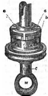
FIG. 8.—Ball Bearings of Neptune Log.
