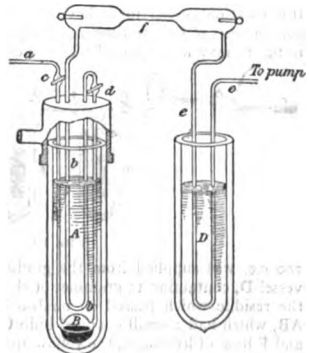
FIG. 9.—Apparatus for continuous Spectroscopic Examination.
