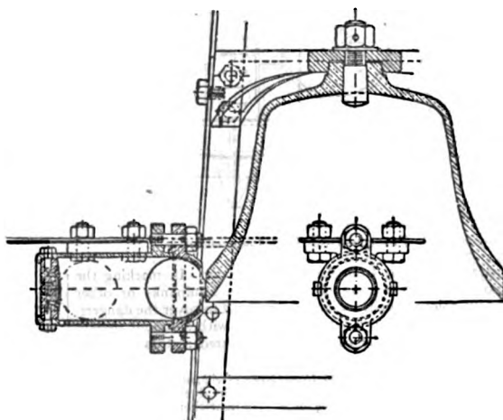
FIG. 52.—Buoy Bell.
