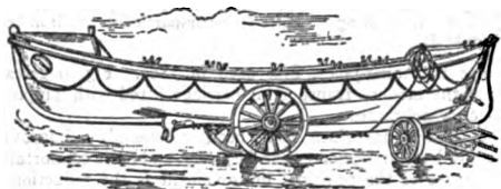
FIG. 1.—The 33-ft., Double-banked, Ten-oared, Self-righting and Self-empting Life-boat (1881) of the Institution on its Transporting Carriage, ready for launching.
