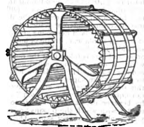
FIG. 10.—Dash Wheel.
