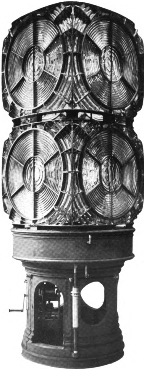
Fig. 54.—Fastnet Lighthouse—First Order Single-Flashing Biform Apparatus.
