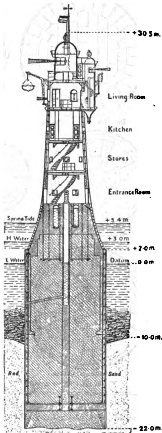
FIG. 21.—Rothersand Lighthouse.
