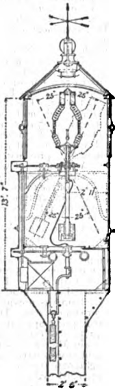
FIG. 48.—Lantern of Sandetti Lightship.
