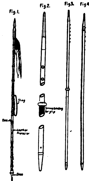
TYPES OF BRITISH AND GERMAN LANCES.
